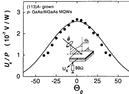
Fig. 2. Photoresponse of 20 p -type (113)A- grown GaAs/AlGaAs QWs normalized by the light power P as a function of the angle of incidence \Theta_0 for right circularly polarized radiation measured perpendicular to light propagation ( T = 300 K, \lambda = 76 \mu\text{m} ). Full line is fitted to Eq. (2) using one y -axis scaling parameter.
