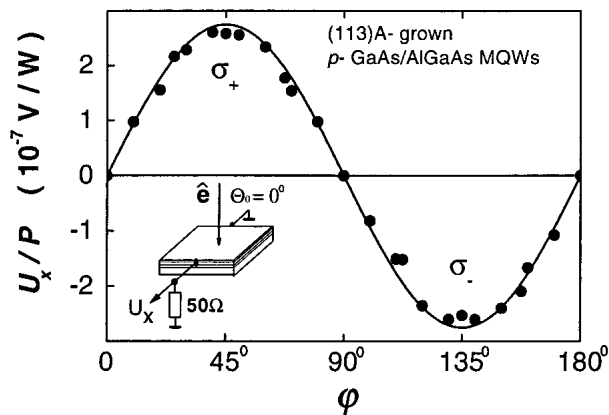
Fig. 1. Photoresponse of p -type (113)A- grown GaAs/AlGaAs QWs structure normalized by the light power P as a function of the phase angle \varphi defining helicity. Measurements are presented for T = 300 K and normal incidence of radiation at \lambda = 76 \mu\text{m} . The current j_x \propto U_x flows along [1\bar{1}0] - direction perpendicular to the mirror plane of the C_s symmetry. Full lines are fitted to Eq. (1) using one y -axis scaling parameter. The inset shows the geometry of the experiment.
