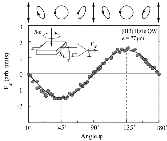
FIG. 1. Helicity dependence of the photoresponse normalized by the radiation power V_x/P in a (013)-grown HgTe QW at room temperature. The signals are obtained at \lambda=77 \mu\text{m} applying pulsed radiation of \text{NH}_3 terahertz laser. The full line is a fit after Eq. (1). The inset shows the experimental geometry. On top of the figure polarization ellipses corresponding to various phase angles \varphi are plotted viewing from the direction toward which the wave approaches.
